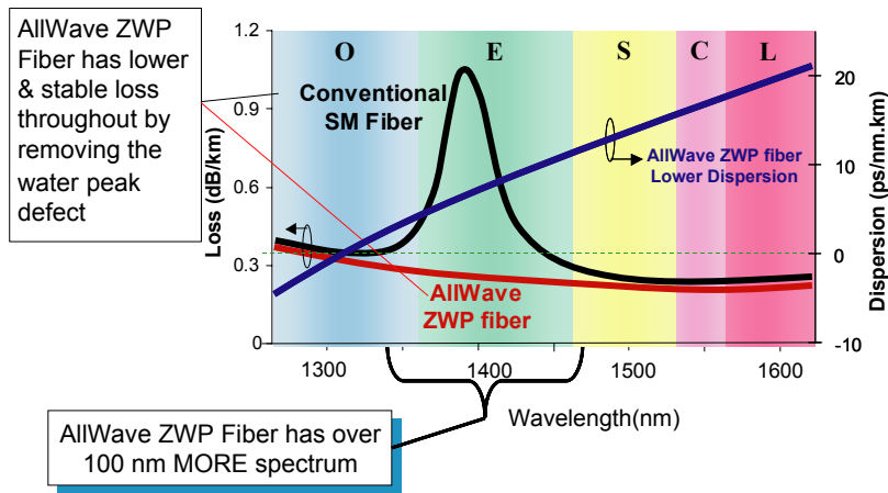
Figure 1. AllWave® ZWP Fiber- Compatible with Conventional Single-Mode fiber, but with More Available Spectrum
