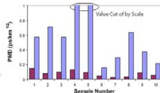
Without OFS PMD Process
